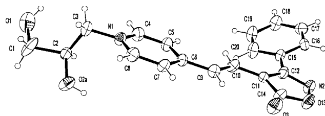
Fig. 2 View of the molecular structure of 5 using 30% probability ellipsoids for non-hydrogen atoms. 20,21 Atom numbering is non-standard (IUPAC) but is concurrent with that used in Table 2.
